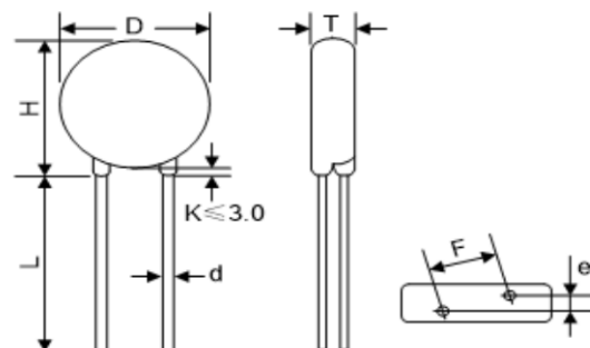
Fig 3. Straight Lead
