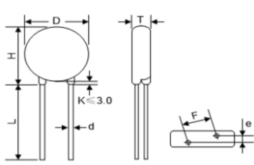
Fig 3. Straight Lead
